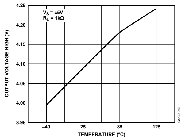
Figure 13. Output Voltage High vs. Temperature at ±5 V
