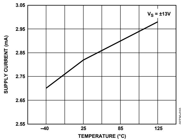
Figure 10. Supply Current vs. Temperature at ±13 V
