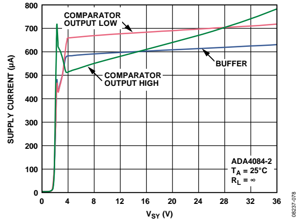
Figure 78. Supply Current vs. Supply Voltage
