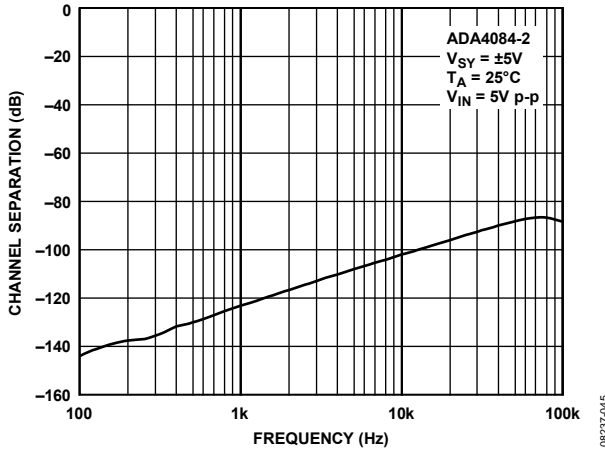
Figure 45. Channel Separation
