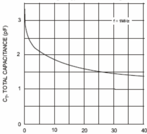
Fig. 3 Typical Capacitance
