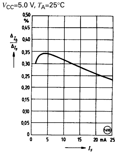
Figure 15. Small Signal Transfer Ratio vs. Forward Current
