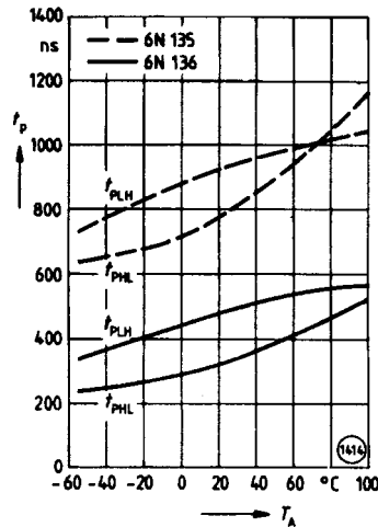
Figure 18. Delay Times vs. Ambient Temperature I_F=16\text{ mA}, V_{CC}=5.0\text{ V}, R_L=4.1\text{ k}\Omega , SFH6136: R_L=1.9\text{ k}\Omega
