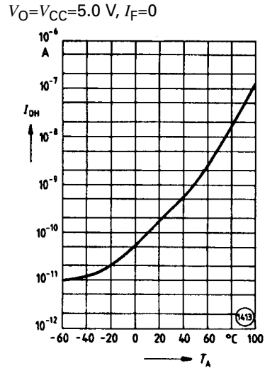
Figure 17. Output Current (high) vs. Ambient Temperature
