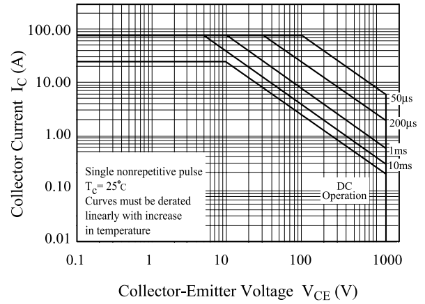
Fig 14. SOA Characteristics
