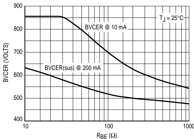
Figure 10. Resistive Breakdown
