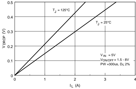
Figure 1. V_{DROP} Versus I_L at V_{IN} = 5\text{V} .
