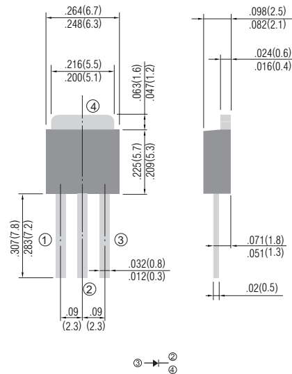
TO-251AB
