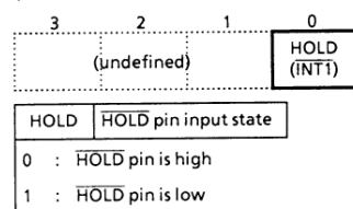
Hold operating mode status register (Port address: IPOE)
